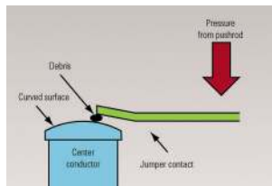
A piece of small debris is stuck on the surface of center conductor
