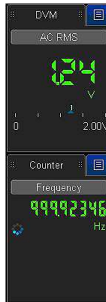
Figure 27. DVM and counter takes advantage of separate signal paths to provide measurements without a trigger, while still using the scope probes.
