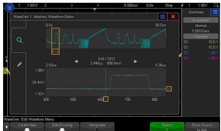
Figure 26. Optional arbitrary waveform generator provides easy access to stimulus. The integrated arbitrary waveform generator makes capturing, modifying and replaying signals simple.
